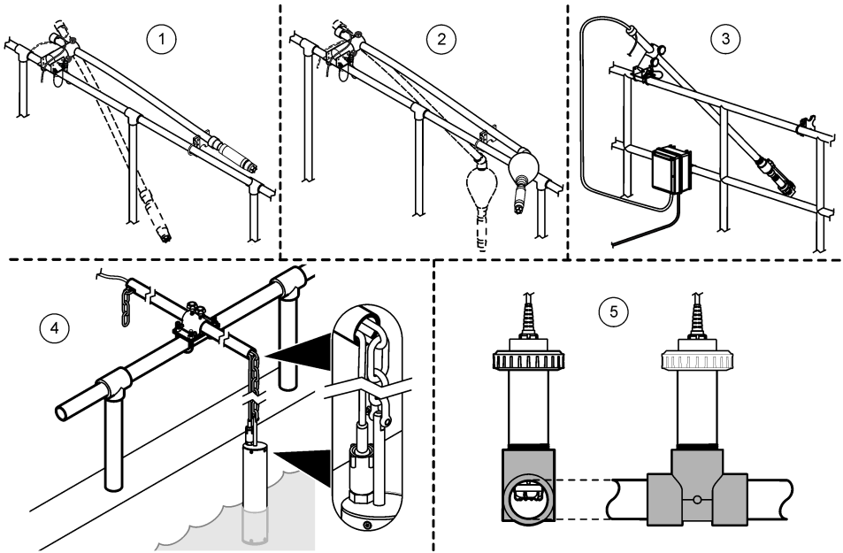
Figure 3 Installation options
