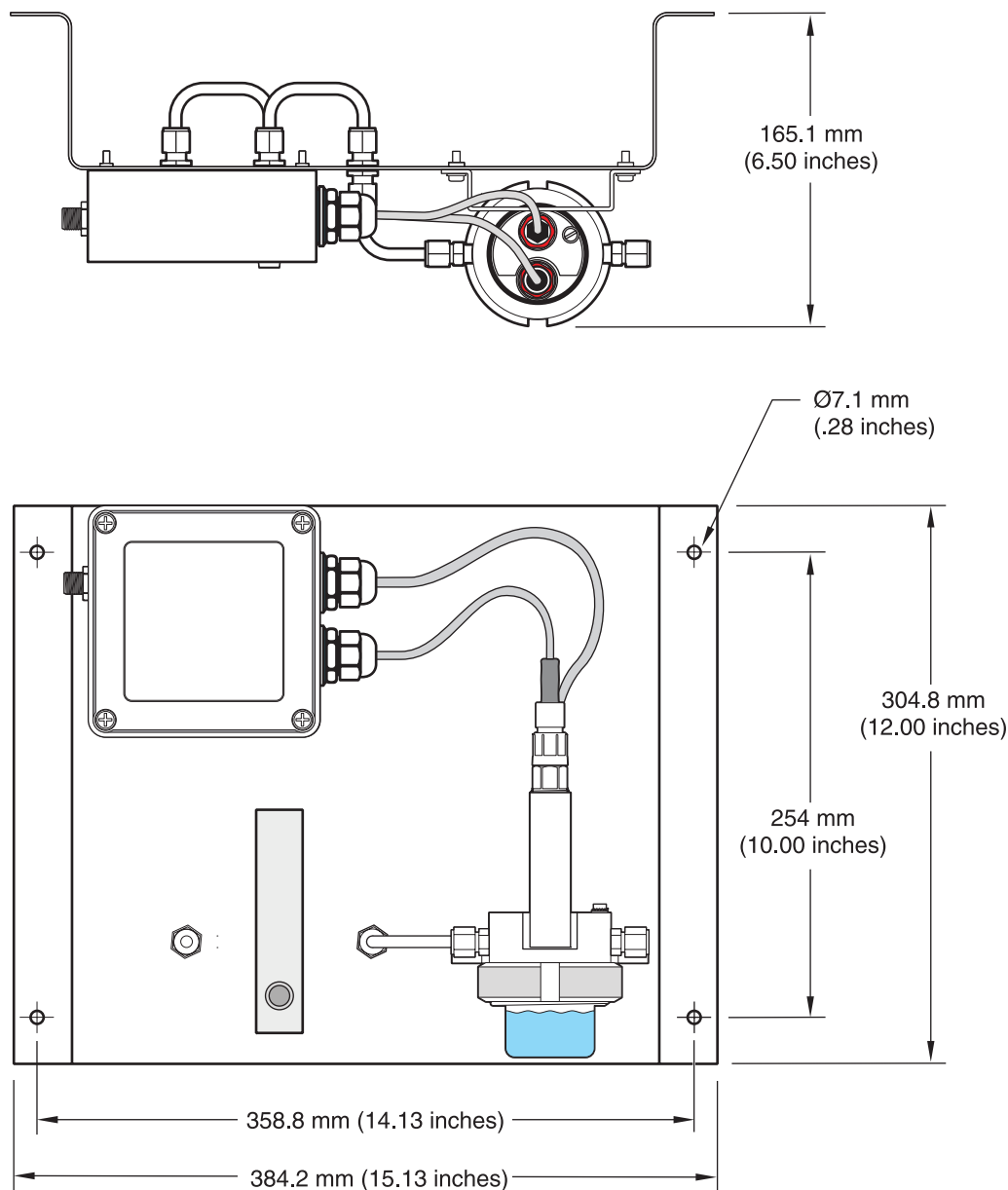
Figure 1 Panel Mounting Dimensions
