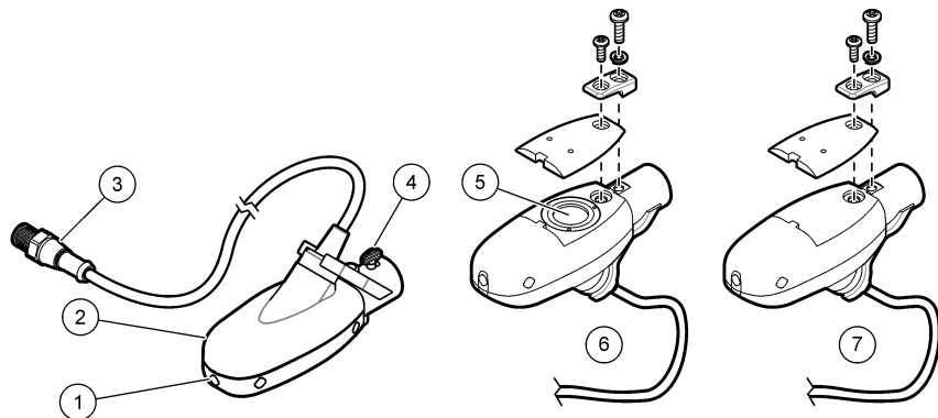
Figure 2 Sensor components
