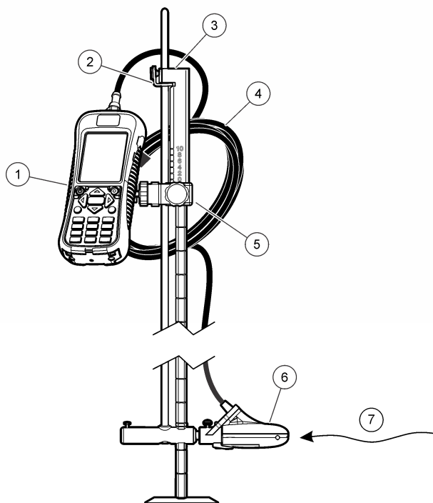
Figure 1 Assembled components
