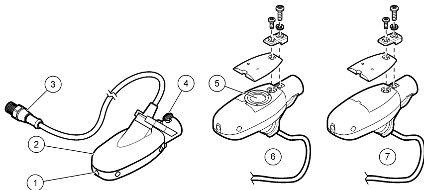
Figure 2 Sensor components
