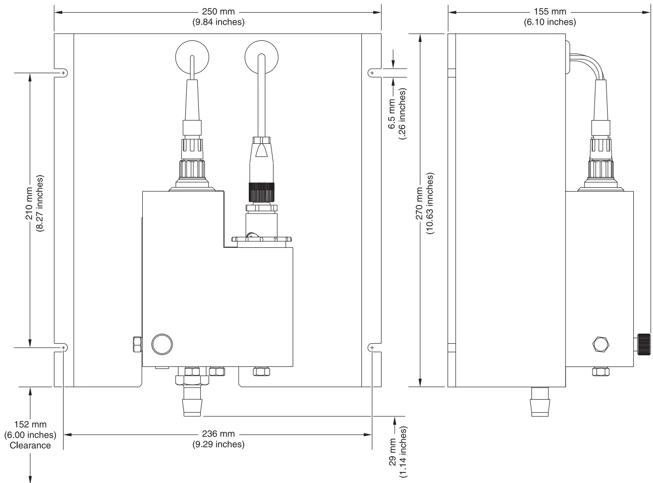
Figure 3 Analyzer Dimensions
