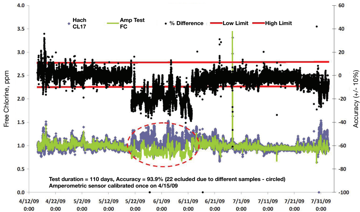
Figure 19 – Free chlorine sensor in pre-tank application (two sampling points per Fig. 16)
