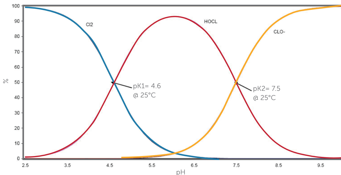
Figure 1 - Free Chlorine Dissociation Curve
