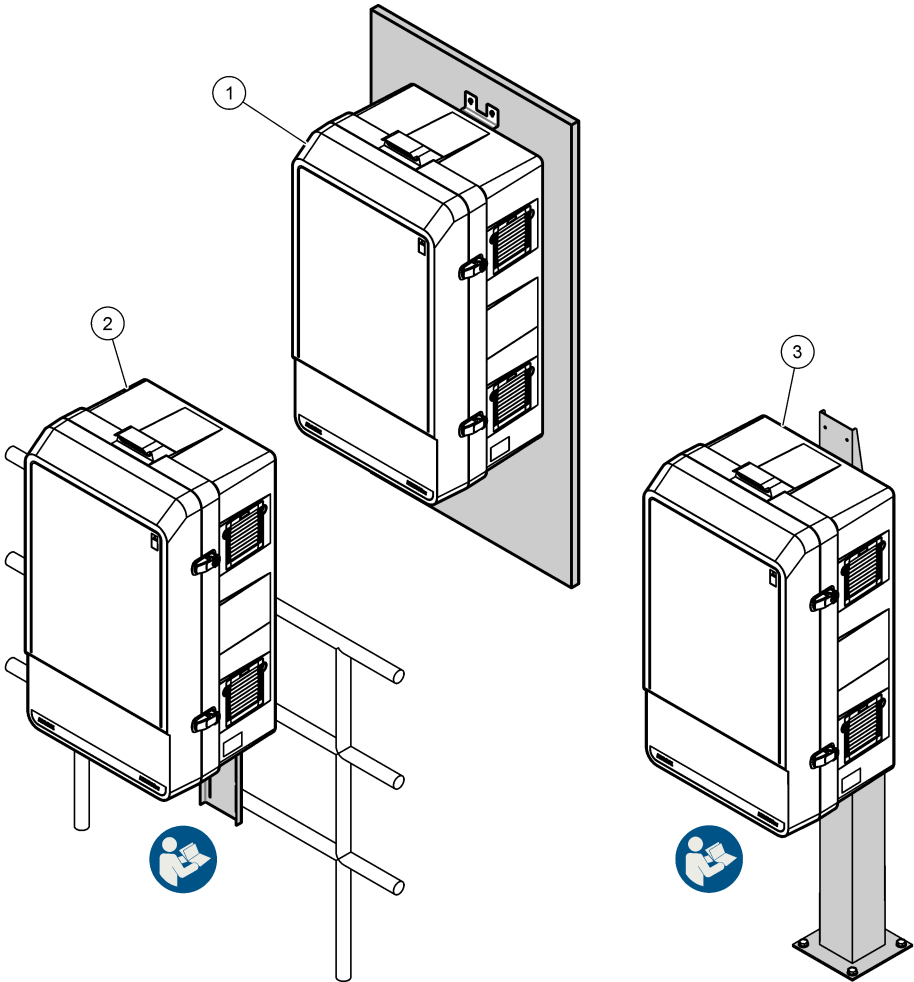
Figure 5 Installation options
