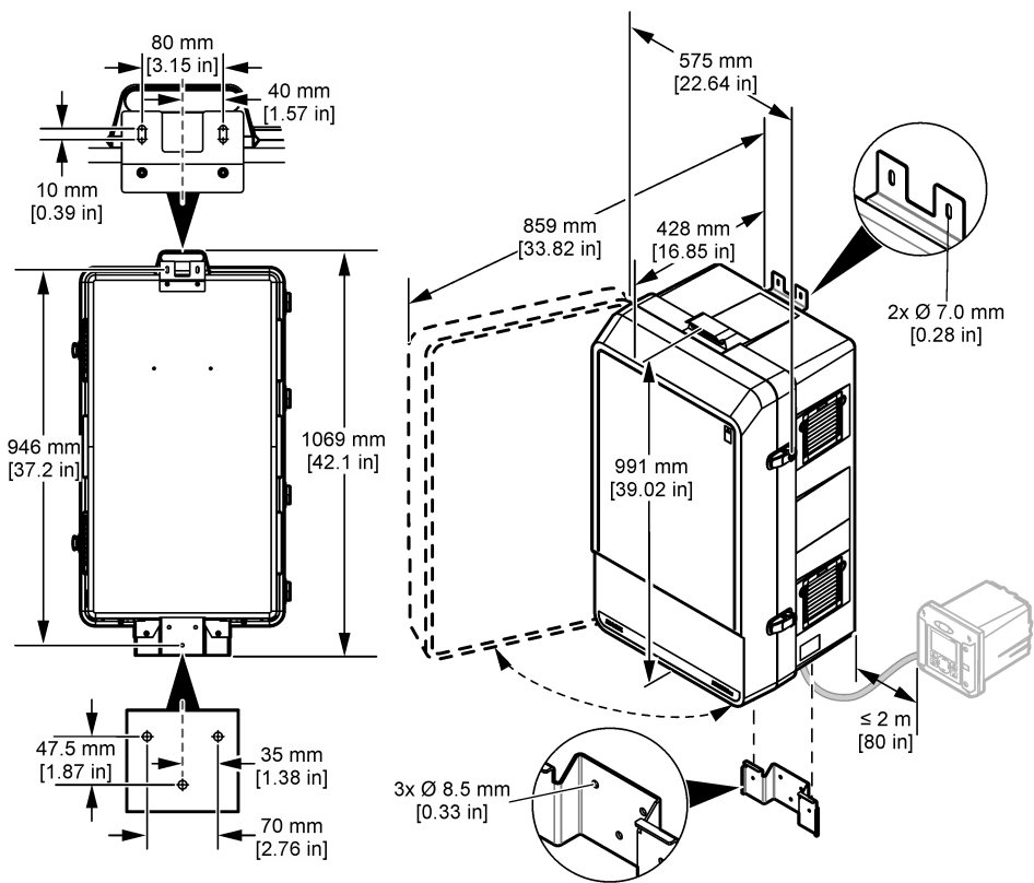
Figure 7 Wall mount
