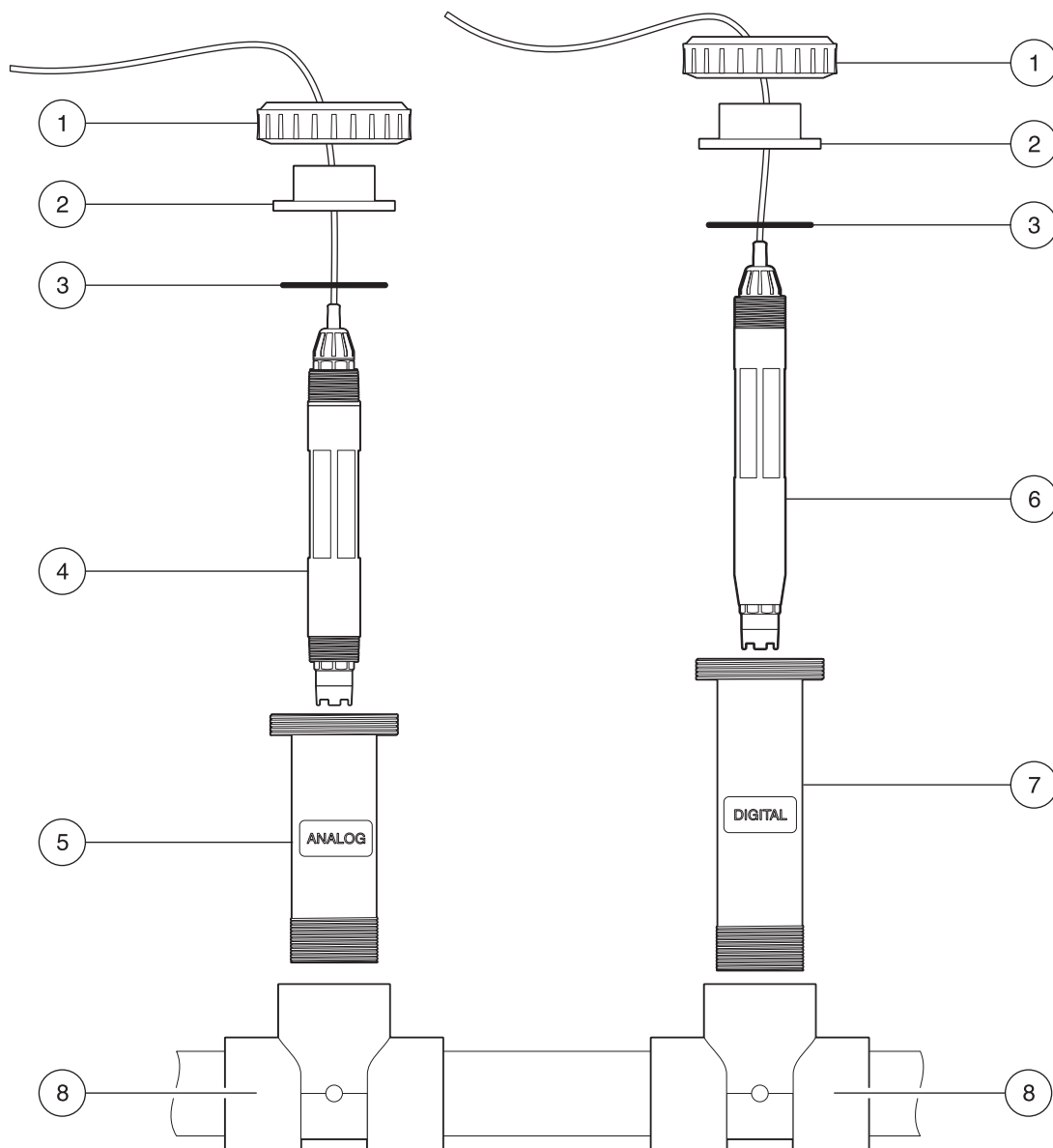
Figure 2 Assembling the union mount hardware
