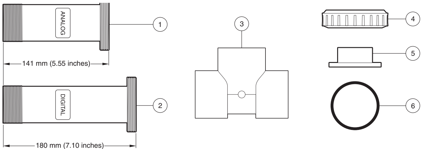
Figure 1 Flow-through union mounting hardware (CPVC shown)
