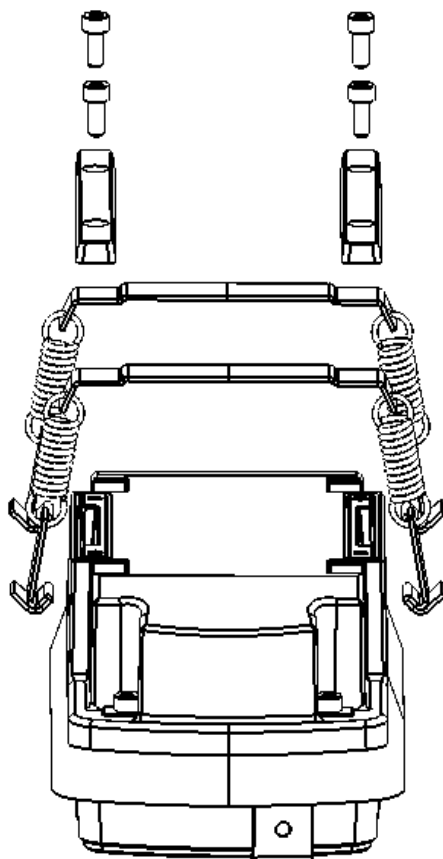
Illustration 9: Placing the clamp straps
