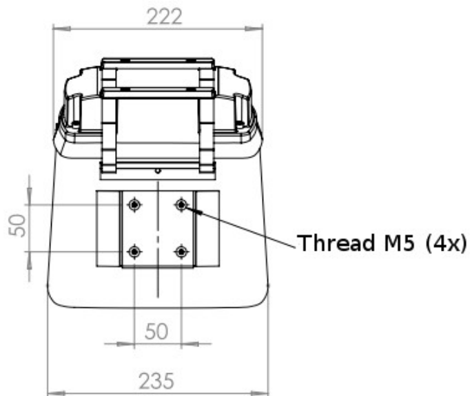
Illustration 27: MARWIS-UMB with short protective housing
