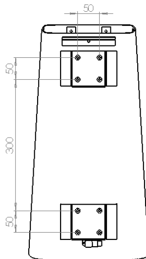
Illustration 29: Long protective housing – back view
