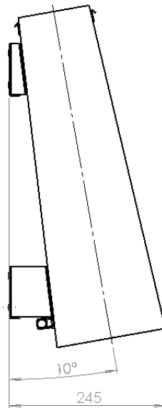
Illustration 28: Long protective housing – lateral view
