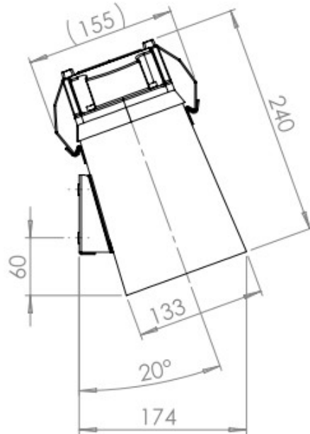
Illustration 26: MARWIS-UMB with short protective housing
