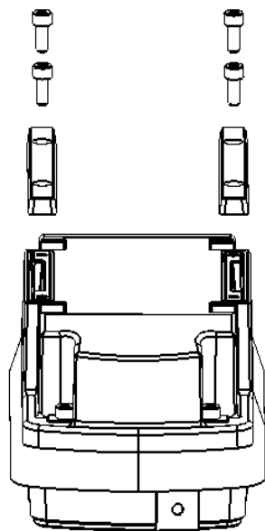
Illustration 6: Preparation for connecting the protective housing
