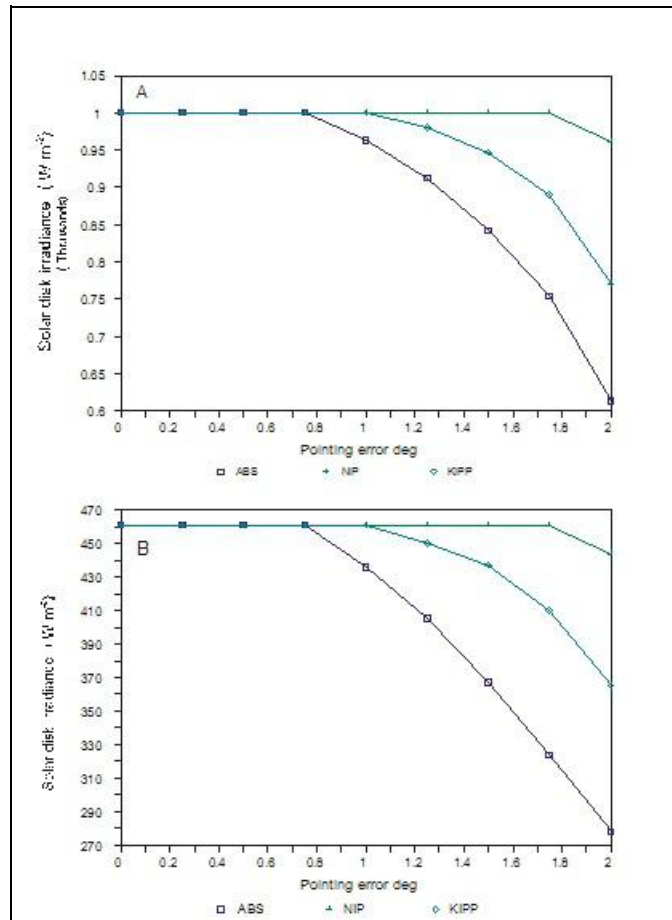
Figure 4.7. The contribution of the solar disk to the irradiance of pyrheliometric sensors depending on the pointing error. (A) Case of mountain aerosol and 60^\circ solar elevation. (B) Case of continental aerosol and a 20^\circ solar elevation. (Calculations and graph courtesy of G. Major)
