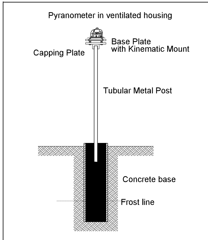
Figure 3.2. Simple post mount in concrete base.
