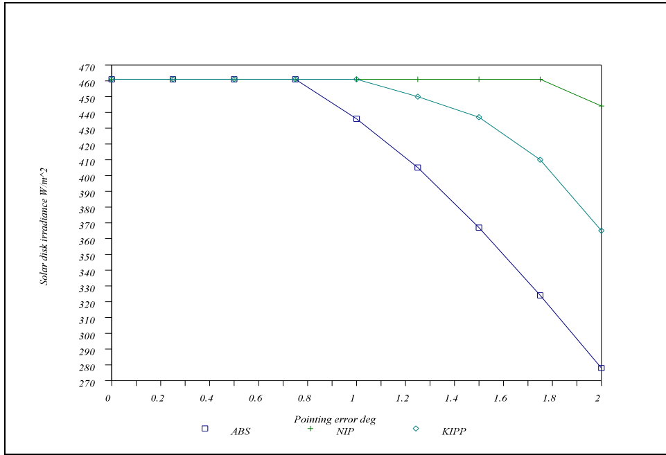
Figure D 1.3. Same as Fig. D 1.2 except the case is for continental background aerosol and 20 degrees solar elevation.
